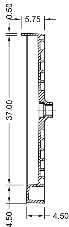
SECTION B-B
