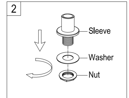
2. Remove washer and nut from soap dispenser sleeve.
