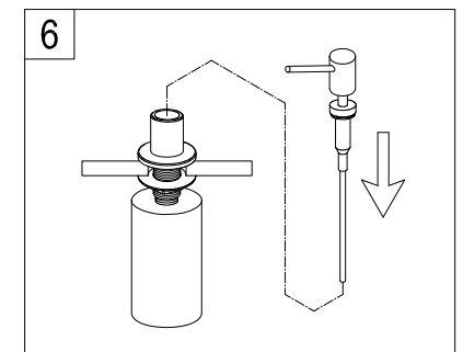
6. Put the pump nozzle and plastic pump into sleeve.
