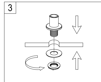
3. Insert soap dispenser sleeve through sink hole and secure with washer and nut.
